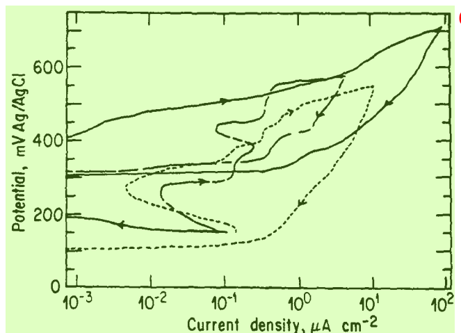
FIGURE 4 — Stepped potentiostatic polarization curves for Alloy 600 (—); Alloy 800 (---); AISI 304 SS (····) in 7.0 \times 10^{-4} \text{ M Cl}^- solutions at 80 C.
