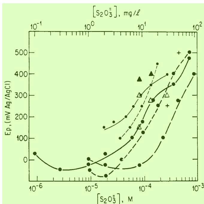
FIGURE 1 — Variations of the pitting potential in 7.0 \times 10^{-4} M \text{Cl}^- solutions at (a) 24 C for Alloy 600 (● — — ●); Alloy 800 (○ — — ○); AISI 304 SS (Δ, ▲, + for repassivating pits, stable pitting and potentiostatically initiated pits respectively); (b) 80 C for Alloy 600 (● — — ●); Alloy 800 (○ — — ○); AISI 304 SS (● — — ●).
